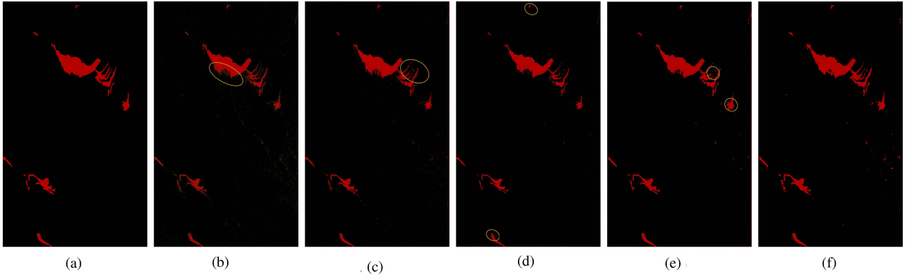
Fig. 21. Results of different methods for Gulf of Mexico Oil Spill Image II. (a) Ground truth. (b) RF. (c) Improved-2D-CNN. (d) Dual-EndNet. (e) DRSNet. (f) MSHFFNet.
