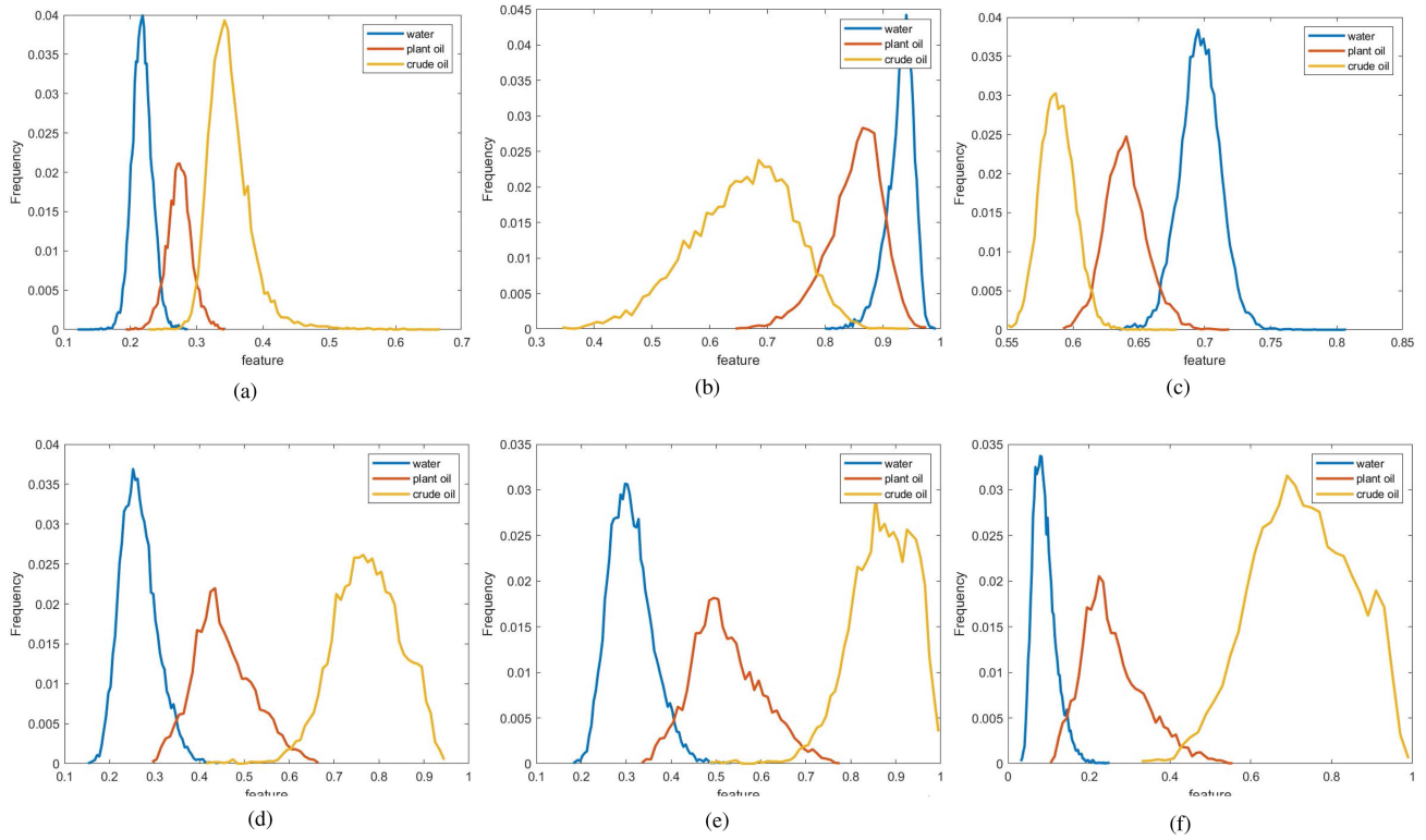
Fig. 9. Plot of PDFs of polarimetric features in selected regions. (a) R_{CO} . (b) \eta . (c) span . (d) H . (e) H_p . (f) H_c .
