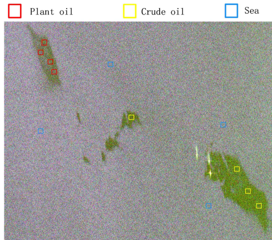
Fig. 3. Sample selection on European North Sea oil spill image.
