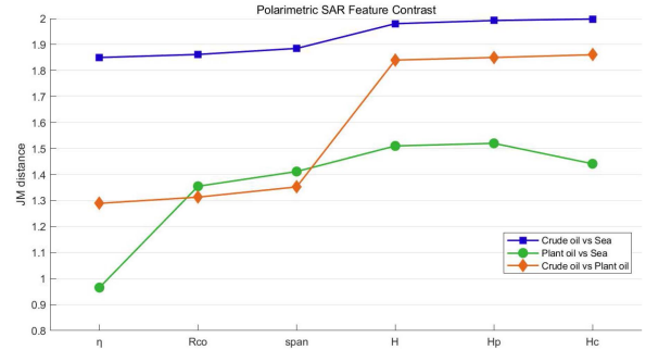
Fig. 7. J–M distance for polarimetric features.
