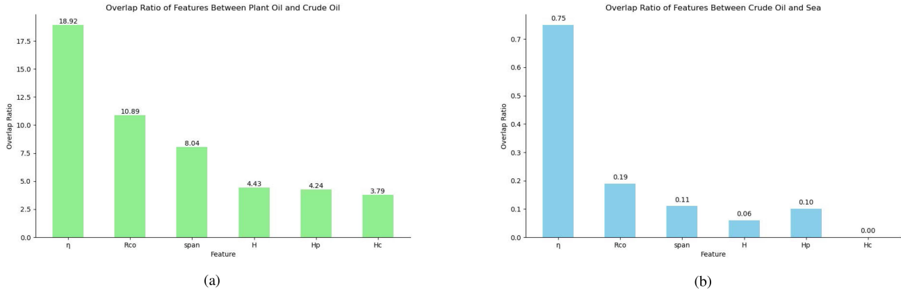
Fig. 10. Overlap area plots for different features. (a) Plant oil versus crude oil. (b) Crude oil versus sea.
