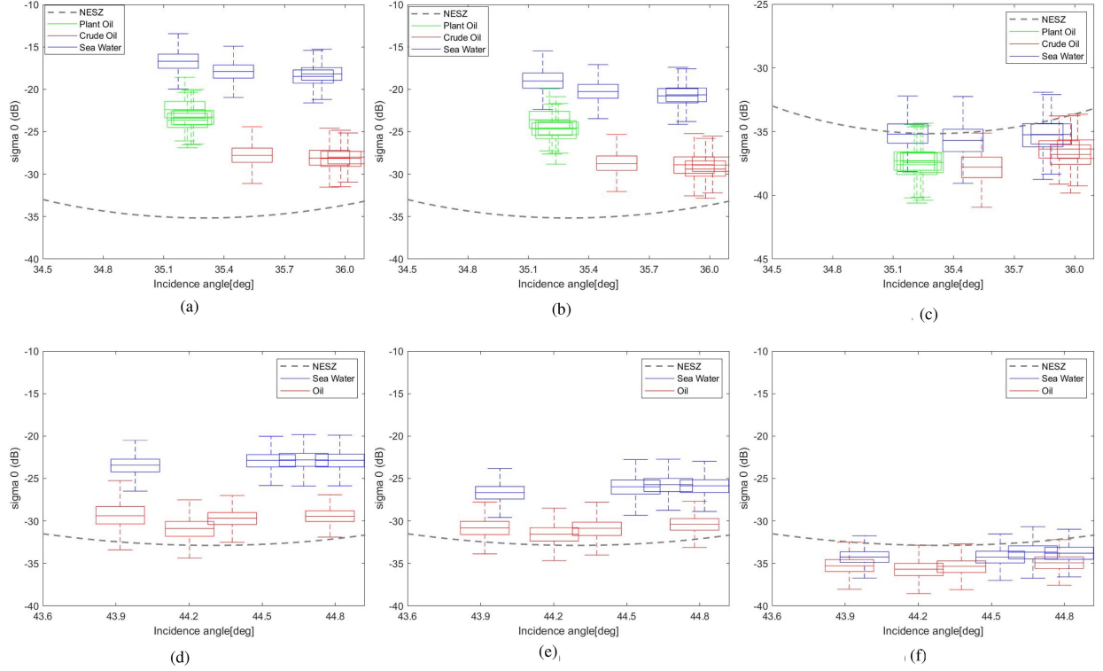
Fig. 24. Signal-to-noise analyses of HH, VV, and VH channels. (a) European North Sea-VV. (b) European North Sea-HH. (c) European North Sea-VH. (d) Gulf of Mexico-VV. (e) Gulf of Mexico-HH. (f) Gulf of Mexico-VH.
