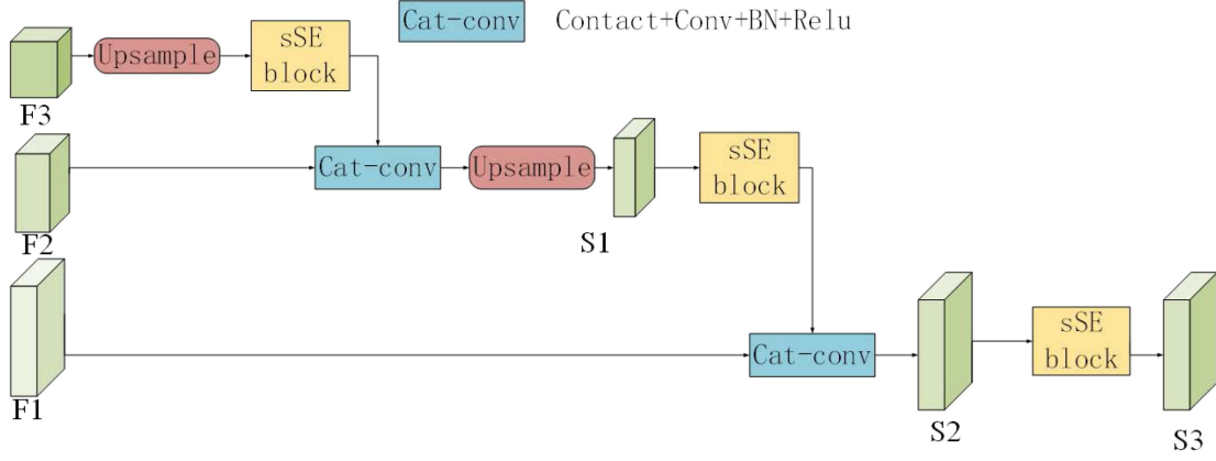
Fig. 16. Structure of the feature fusion module.
